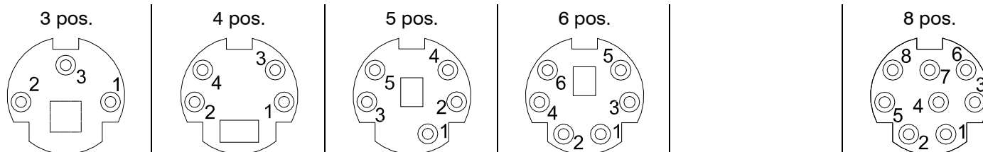
Front View
